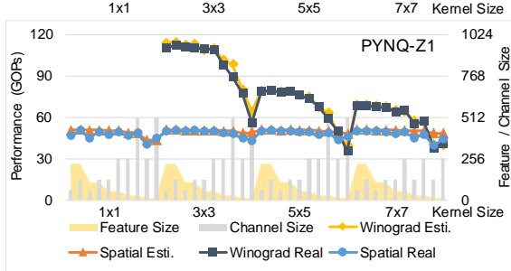
Figure 6: Performance of VU9P and PYNQ-Z1
